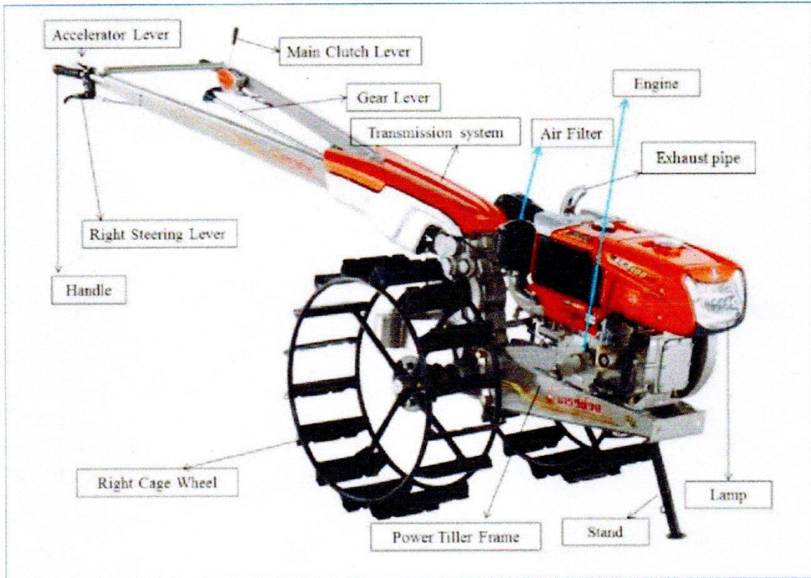
Technical Drawing of Handtractor
